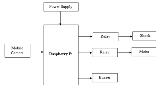
Fig1: Block Diagram
